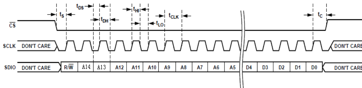
Serial Control Port Write—MSB First, 16-Bit Instruction, Timing Measurements
