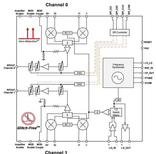
Figure 1. Block Diagram
